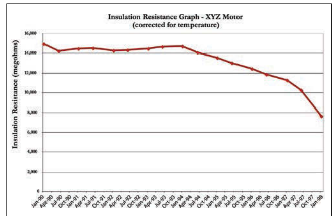
Figure 33: Insulation Resistance Graph Corrected for Temperature
