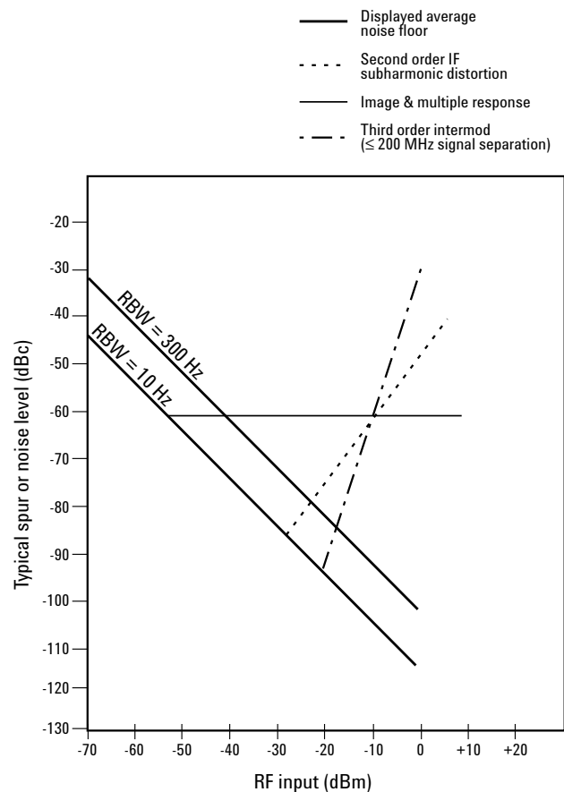
Figure 3. Agilent 11974A System Dynamic Range
