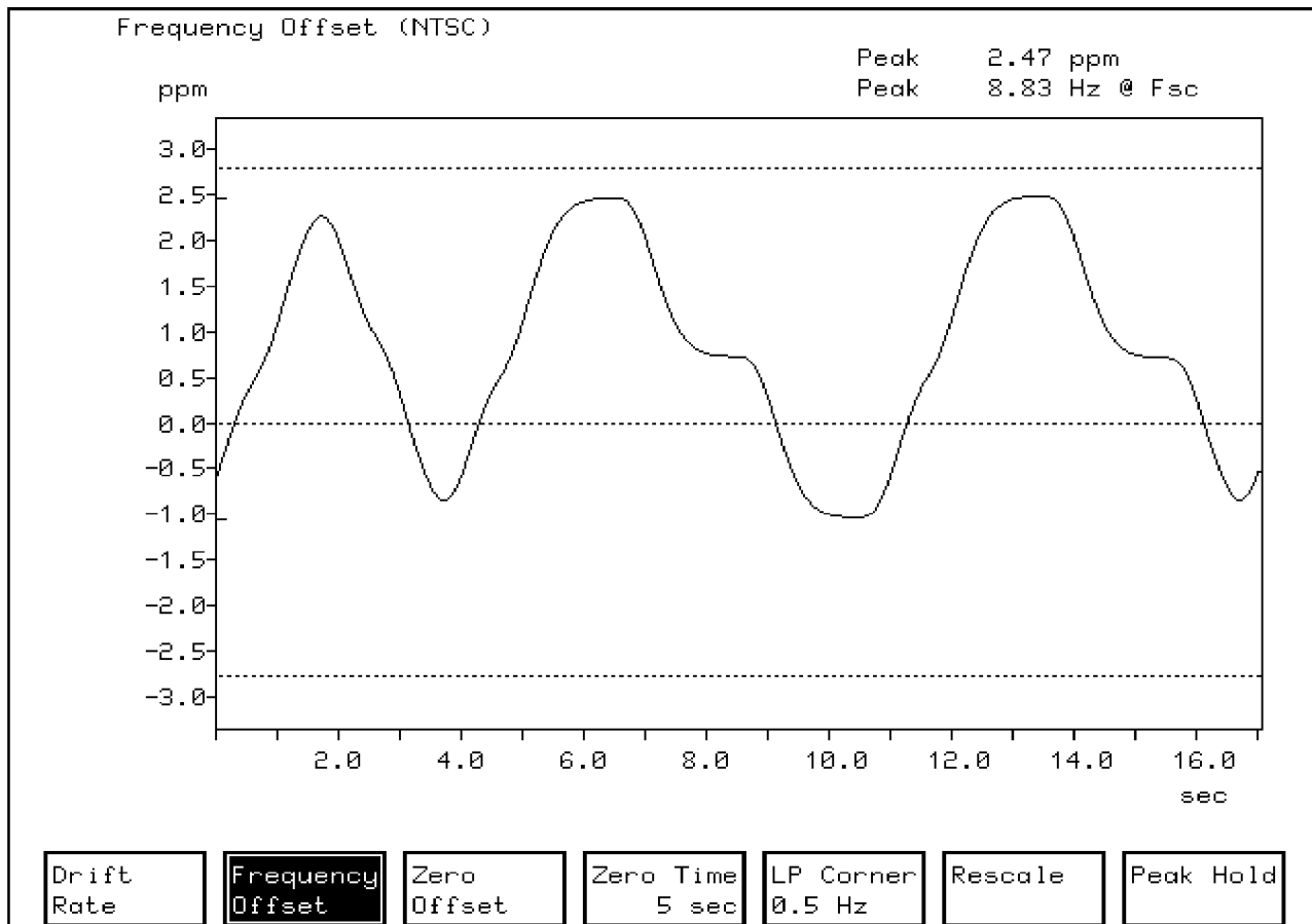
Figure 6: Frequency Offset measurement display
