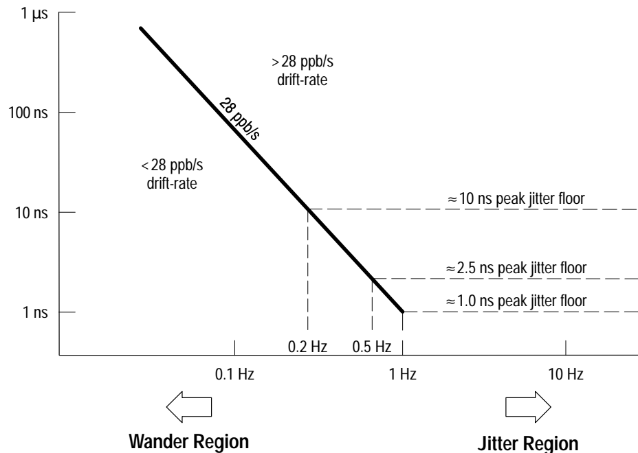
Figure 5: Plot of time error versus frequency accommodation
