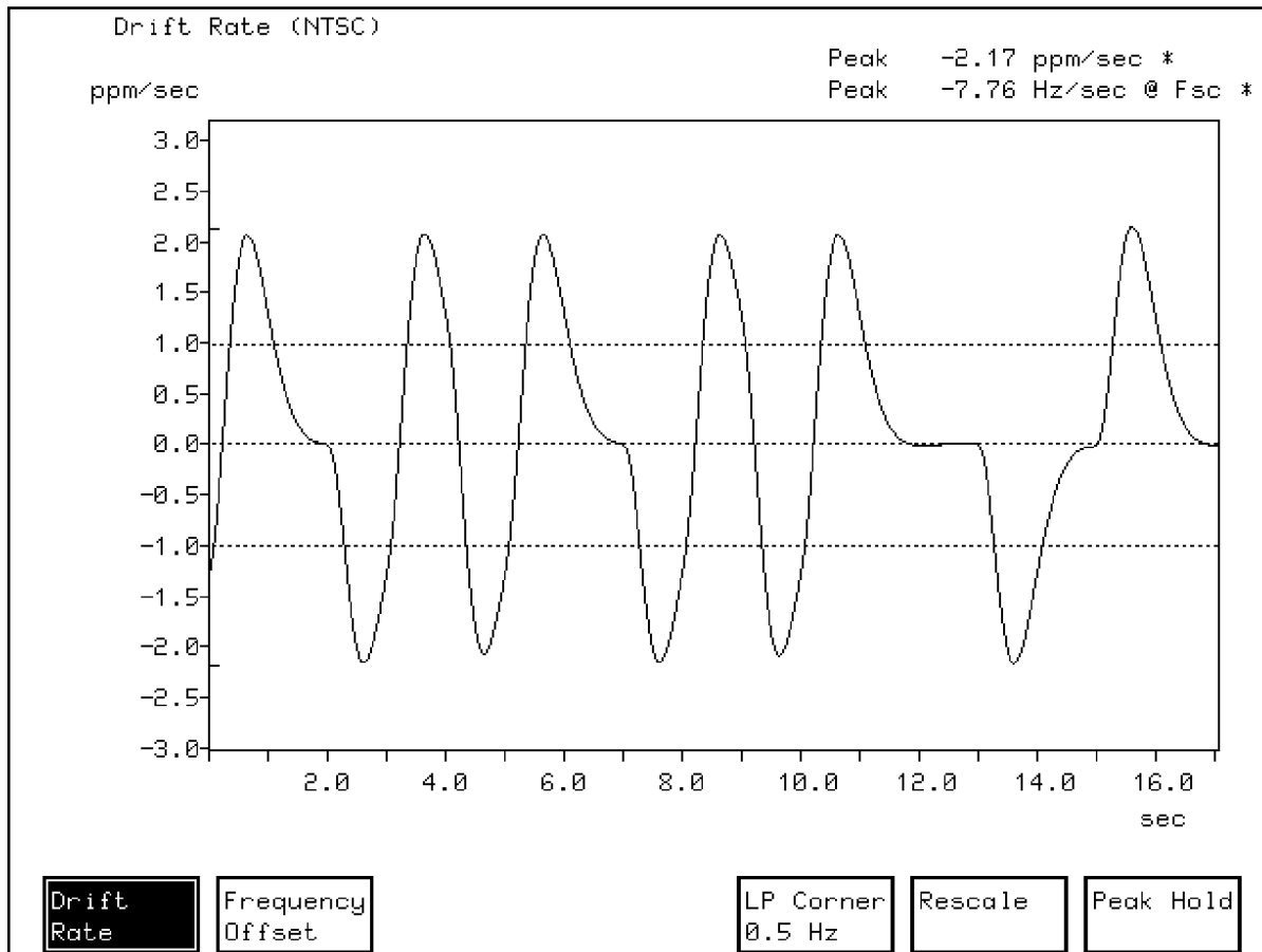
Figure 7: Drift Rate measurement display
