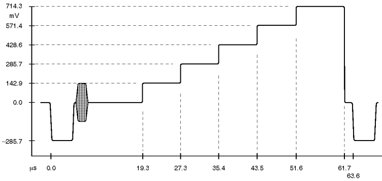
Figure 35: NTSC 5-Step Staircase (Gray Scale)
