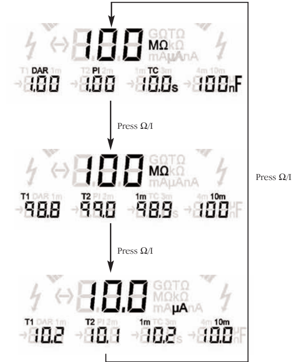
Figure 1 - The result of an insulation resistance test (IR)
