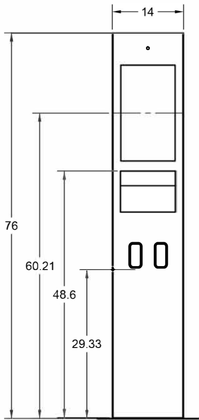
UPRIGHT DIMENSIONS IN INCHES
