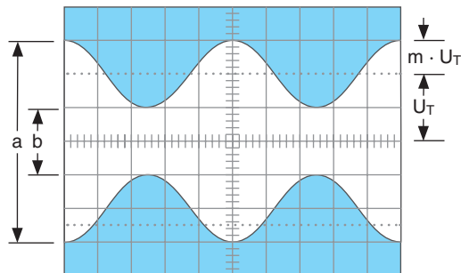
Picture 2: Amplitude modulated hf. F = 1 MHz, f = 1 kHz, m = 50 %, U T = 28,3 mV rms Set the scope controls as follows in order to display the picture 2 signal:
