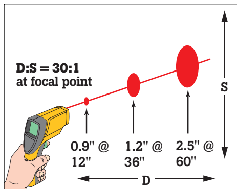
Use the Fluke 66 within 5 m (15 ft.) of the intended target. At greater distances, the measured area will be larger (approximately the distance divided by 30).
