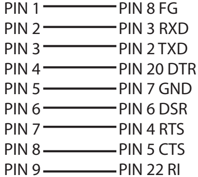
9-PIN to 25-PIN Adaptor
