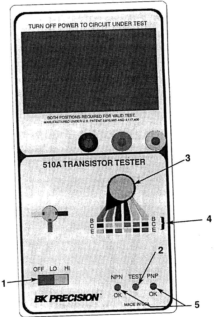
Fig. 1. Front panel showing controls and indicators.
