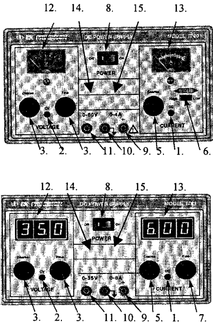
Figure 1. Front Panel Controls (1744A top - 1745A bottom)
