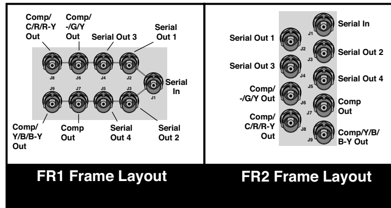
FR1 and FR2 BNC Connector Assignments, R10CE Card Module
