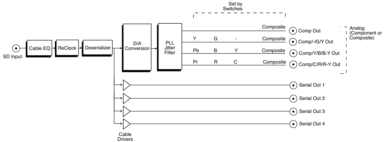
R10CE Monitoring Digital DA, Simplified Block Diagram
