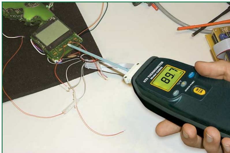
Precise RTD temperature sensor allows for accurate temperature measurement at specific points on the surface of electronic circuits.
